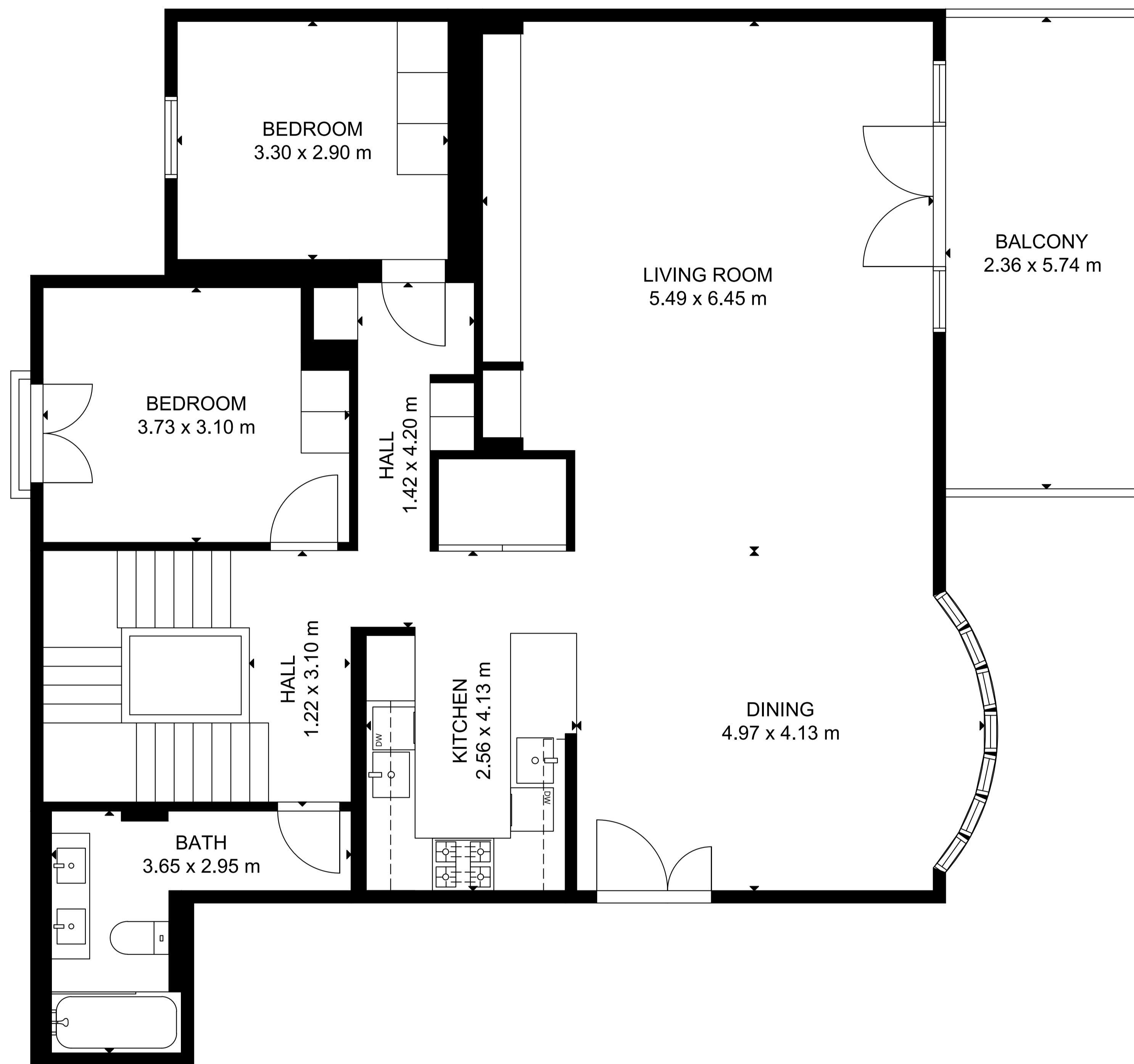
FLOOR 2
