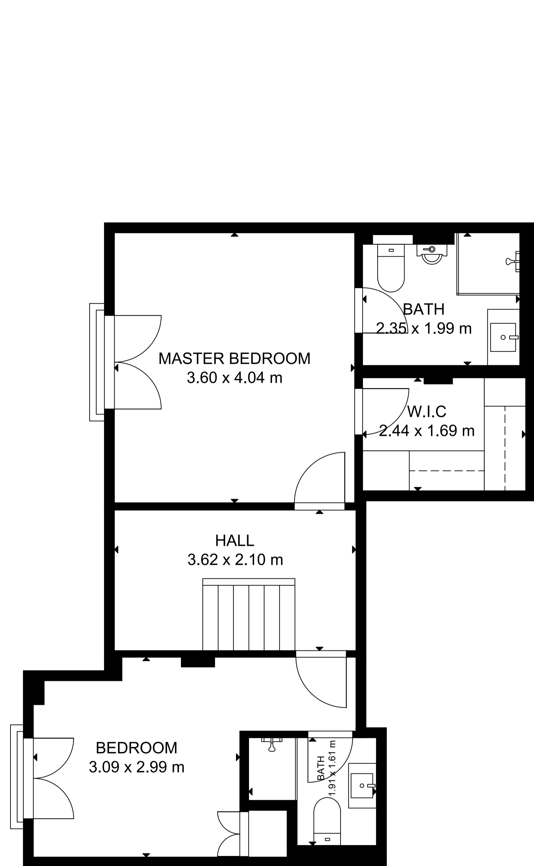
FLOOR 1
