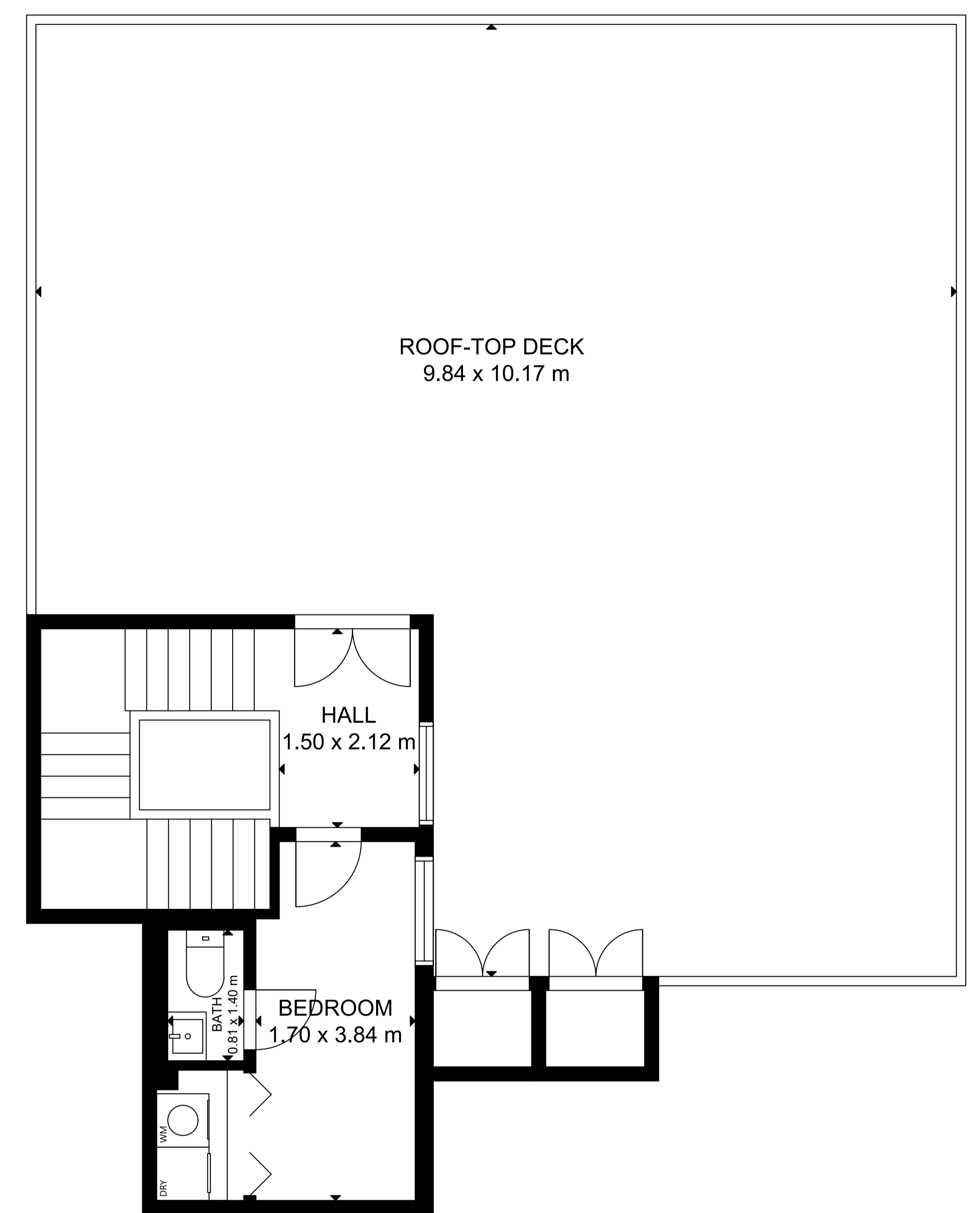
FLOOR 3
