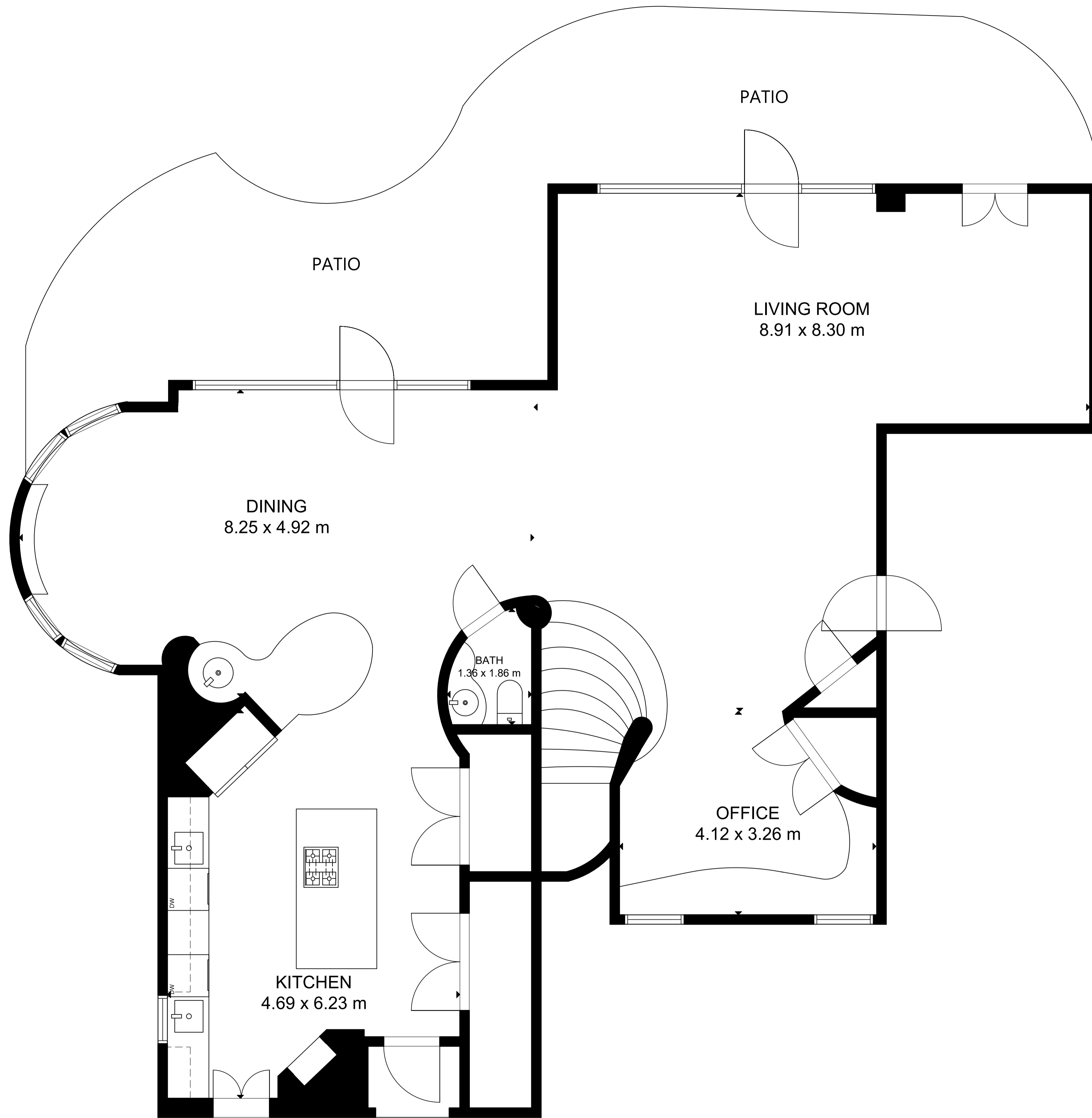
FLOOR 1
